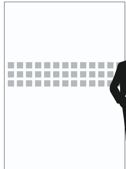
Glass shown as 60" x 84" 3" squares with .5" space
